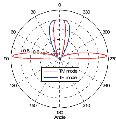
Fig.5. Emittance for resonance frequencies \omega=0.6815 and \omega=1.315 .
